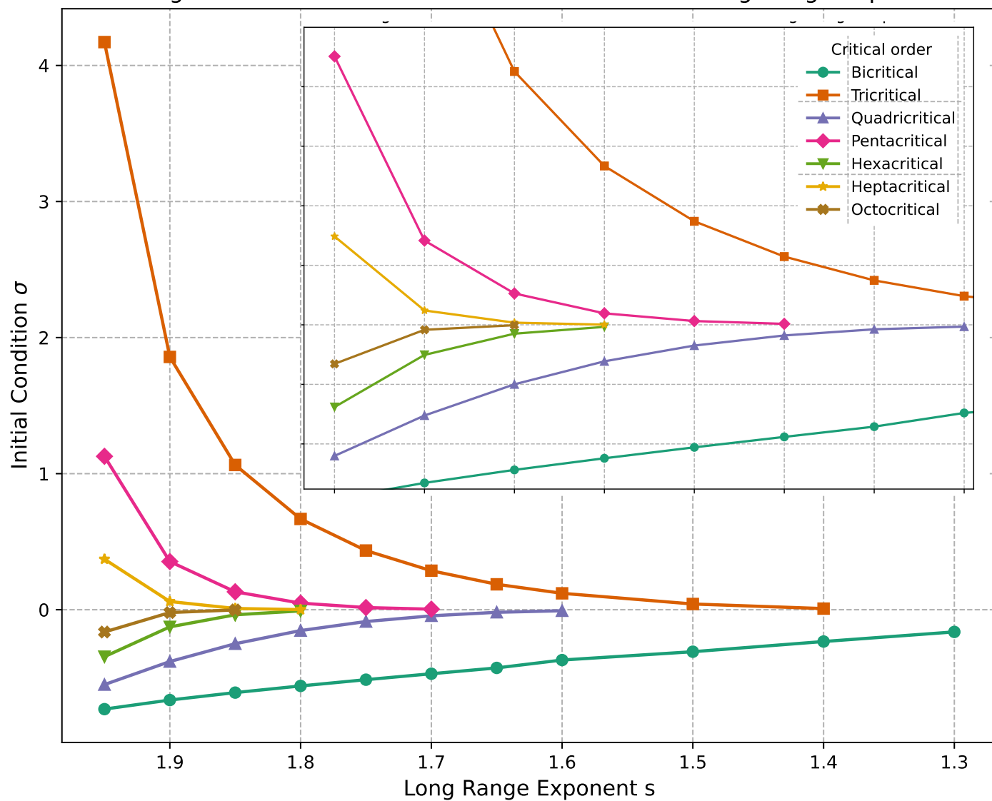
Emergence of Multicritical Solutions as function of Long Range Exponent
